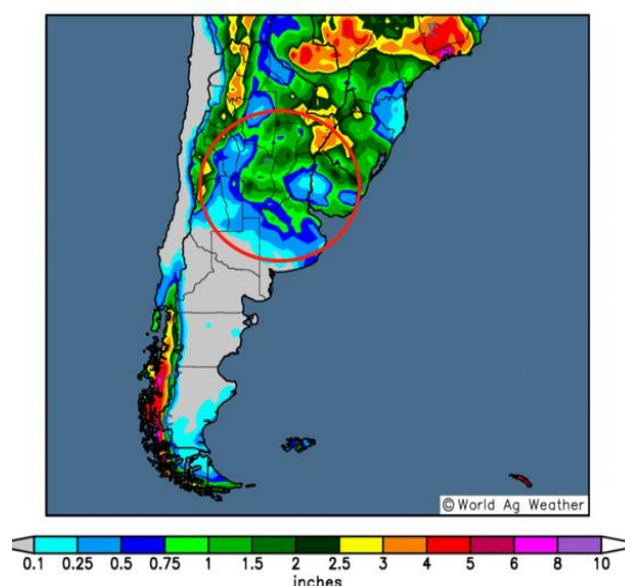
GFS High-Resolution Precipitation Forecast Days 1-7: 00UTC 11 Feb 2023 – 00UTC 18 Feb 2023 Model Initialized 00UTC 10 Feb 2023
