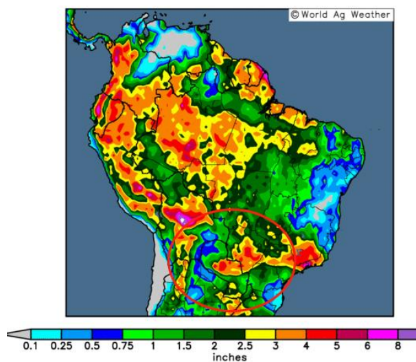
GFS High-Resolution Precipitation Forecast Days 1-7: 00UTC 11 Feb 2023 – 00UTC 18 Feb 2023 Model Initialized 00UTC 10 Feb 2023
